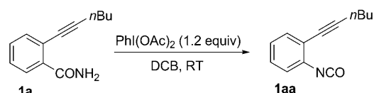
Scheme 3. Hofmann-type rearrangement of 2-(1-hexynyl)benzamide 1a .
